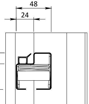
DETAIL G
