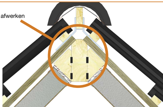
Nokdetail
