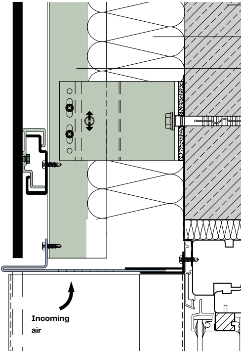
Lintel A101
