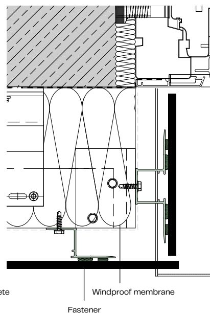
Window reveal A104
