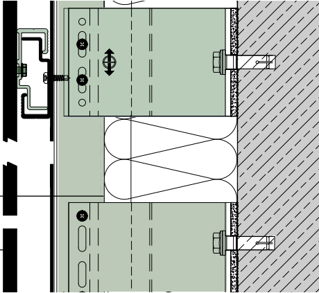
Horizontal joint A110
