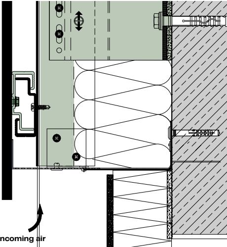
Joint with base A103
