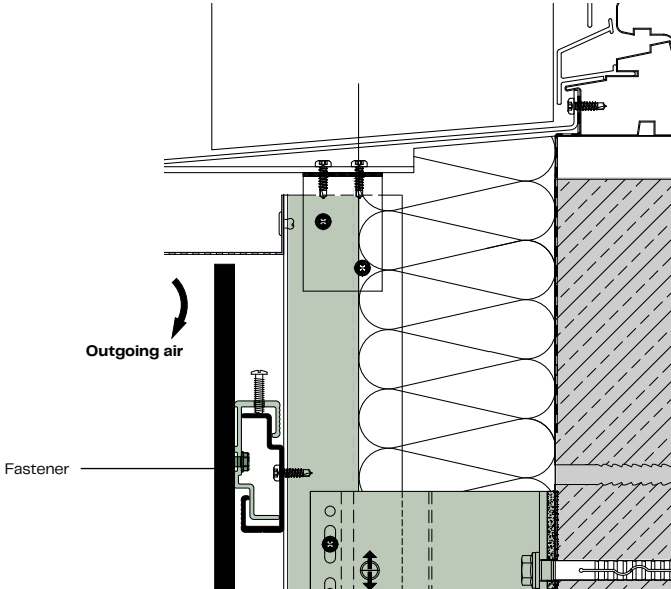
Joint with window sill A102
