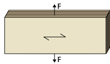
F f_{t,90,edge} Edgewise, perp. to grain ♦♦
