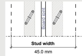
Schematic diagram of the board joint
