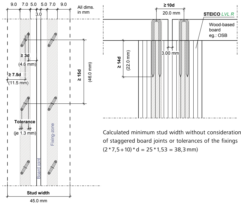
Staple geometry e.g. Haubold KG 700
