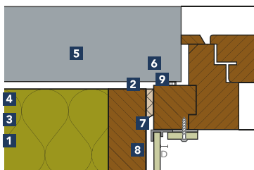
Detail 1-302
