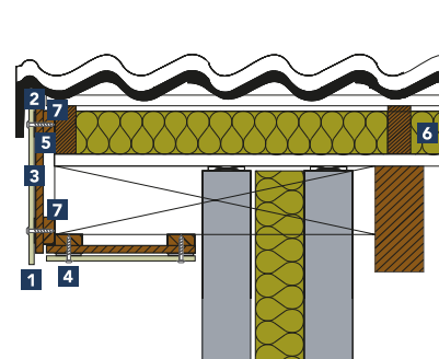
Detail 1-511
