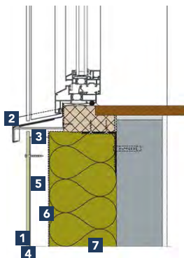
Detail 1-361
