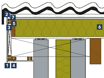
Detail 1-509
