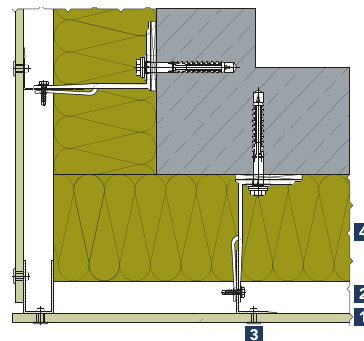
Detail 2-201B
