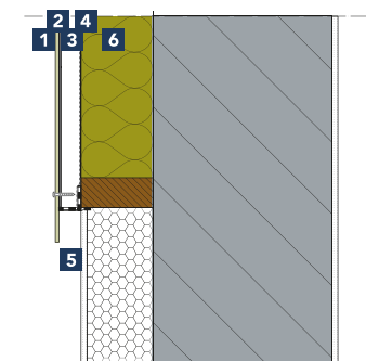
Detail 1-275
