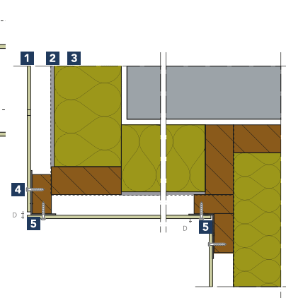
Detail 1-201
