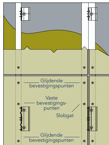
Detail 2-103
