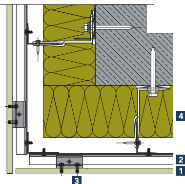
Detail 2-205
