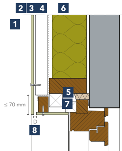
Detail 1-351
