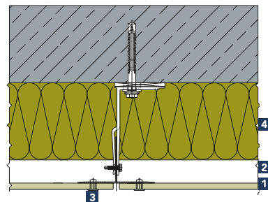
Detail 2-200B
