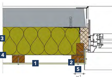
Detail 1-307
