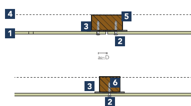
Detail 1-200
