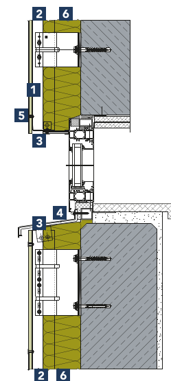
Detail 2-350
