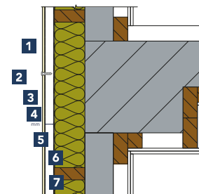
Detail 1-654
