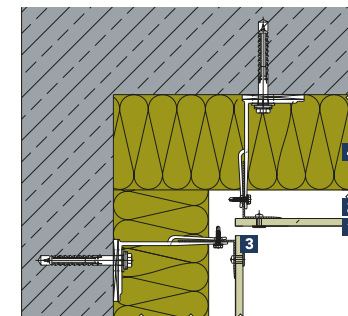
Detail 2-203B
