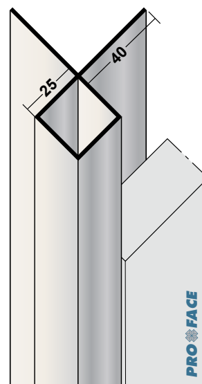
Proface®-CORNEX C250M-A
