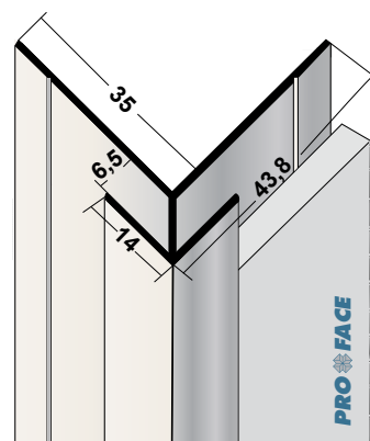
Proface®-CORNEX C65U-A
