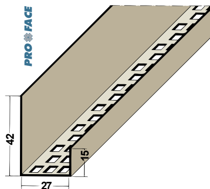
Proface®-VENTILEX VX270-P
