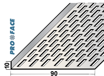
Proface®-VENTILEX VX900T-A
